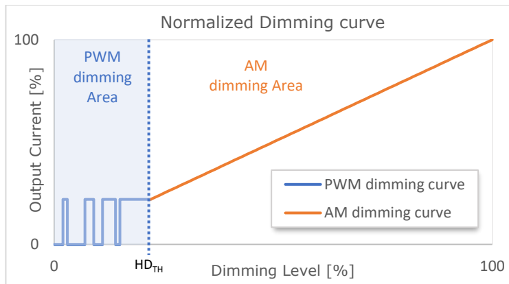
Figure 8: Normalized Dimming curve
